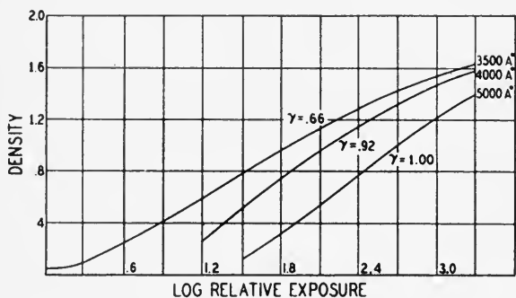
FIG. 3. Variation of gamma with wavelength for E.K. 1359 emulsion.
